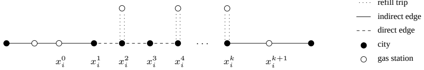
Fig. 1. Decomposition of the solution into strands
