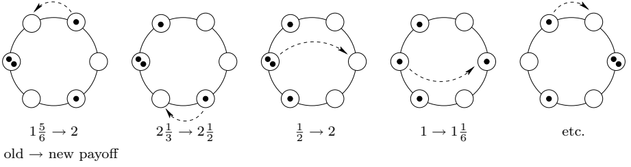
Fig. 2. The best response dynamic does not converge on this graph
