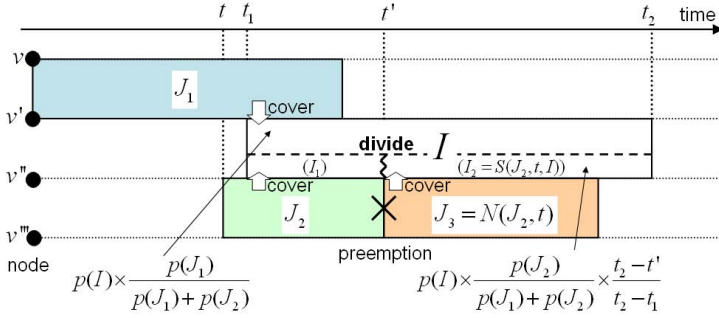
Fig. 1. Example of dividing
