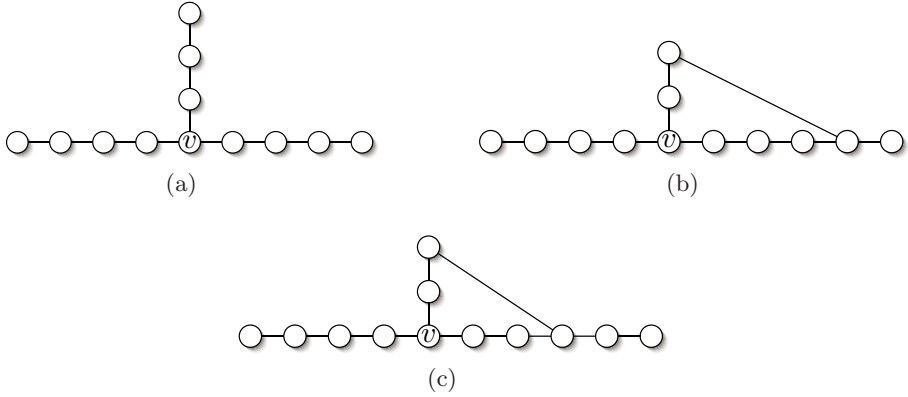
Fig. 1. Examples of Corollary 1 for (6, 9) -coloring. The graphs of 1(a), 1(b) cannot be (6, 9) -colored because |G_v^3| = 10 ; the graph of 1(c) is (6, 9) -colorable because |G_v^r| \leq 2r + 3 for all r \leq 3 .
