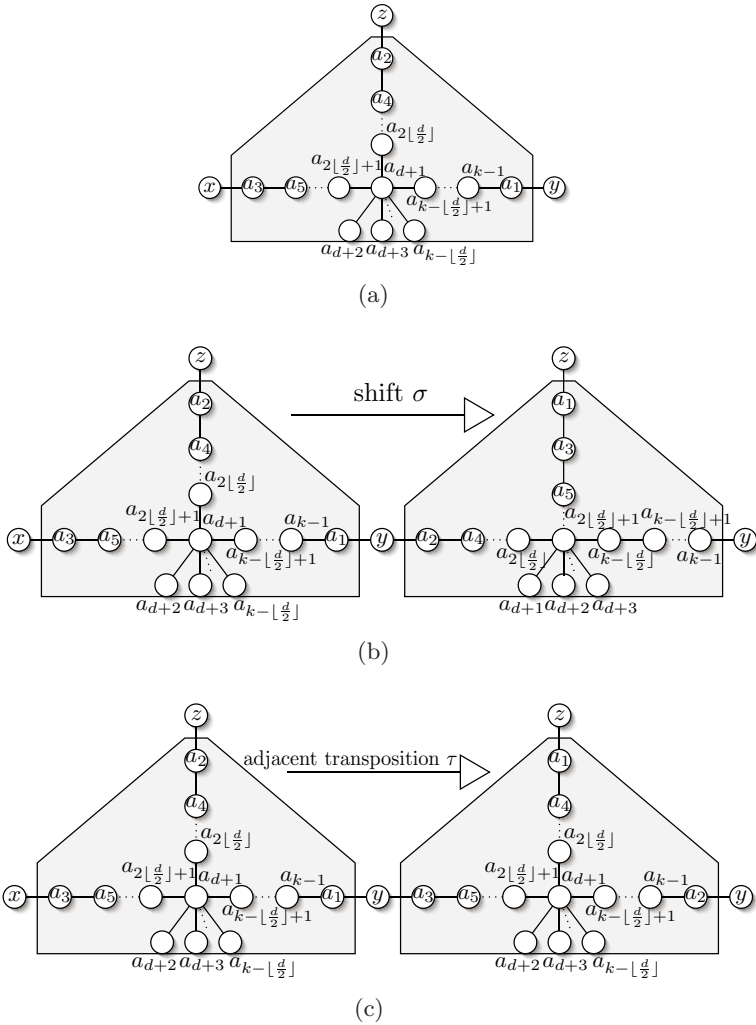
Fig. 4. 4(a) The set A for the basis of the permutation group for odd d . The same labeling can be used for even d , ignoring the center vertex. 4(b) The shift operator \sigma . 4(c) The adjacent transposition operator \tau .
