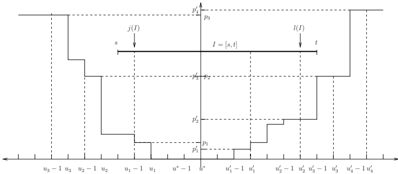
Fig. 1. \epsilon -relative pricings w.r.t. to [u^* - 1, u^*] : To the left is the plot of p([u-1, u^*]) for u < u^* , and to the right is the one for p([u^*, u]) for u \geq u^* . The indices j(I) and l(I) for a given interval I = [s, t] are also shown.
