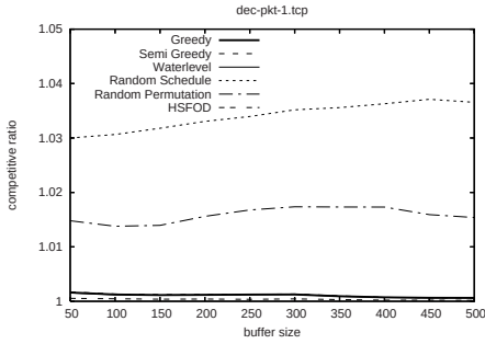
Fig. 3. Comp. ratio, m = 30 & s = 1.0
