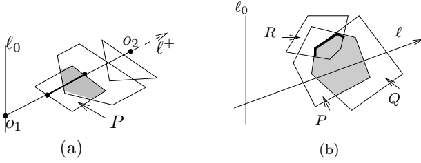
Fig. 3. (a) Query algorithm: case (ii). o_1 and o_2 lie in the same cell of \mathcal{A} , s intersects \bigcap \overline{Front}(C) and o_2 lies out of \bigcap \overline{Front}(C) . (b) Good facets. For the cell C which contains \ell , \bigcap \overline{Front}(C) = P \cap Q . The facets of P \cap Q which are contained in R (bold) are not good and are not intersected by lines in C .
