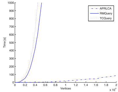
(b) Performance of APR-algorithms on the Internet dag samples
