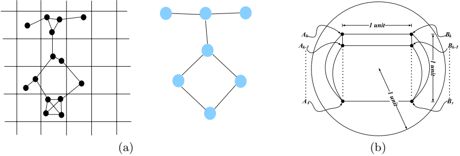
Fig. 1. (a) A realization of a UDG G , partitioned by a grid of \frac{1}{\sqrt{2}} \times \frac{1}{\sqrt{2}} square cells. The cluster graph G[\mathcal{C}] induced by the partition \mathcal{C} is also shown. (b) A bad example for the greedy approach. Each A_i and each B_i is a set of 2^i points. A point in A_i is adjacent to all points in A_j , 1 \leq j \leq k and exactly the points in B_i . The adjacencies for points in B_i are symmetric. Thus the largest clique is A_k \cup B_k and has size 2 \cdot 2^k . Removing this clique leaves sets A_j and B_j , 1 \leq j \leq k-1 intact. Thus the algorithm uses k cliques to cover about 2^{k+2} points, yielding a lower bound of \Omega(\log n) on the size of the clique cover produced by the greedy algorithm.
